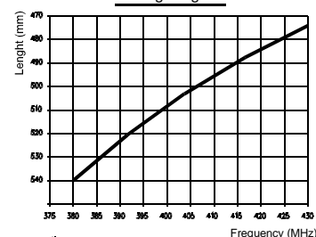
Cutting Diagram
