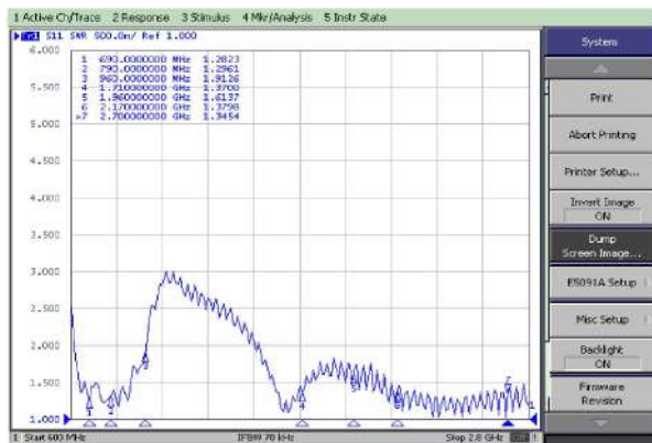
W.S.W.R. Measured with 3000mm cable
