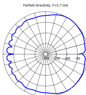
Value with an infinite ground plane
