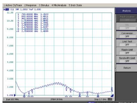
V.S.W.R. Curve
