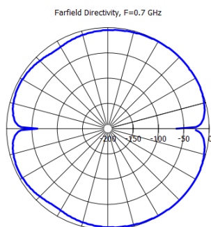
Value with a 60 mm. diameter ground plane
