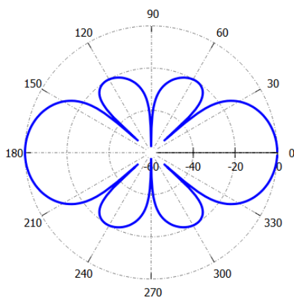
Farfield Directivity 160 MHz - E-plane [dB]
