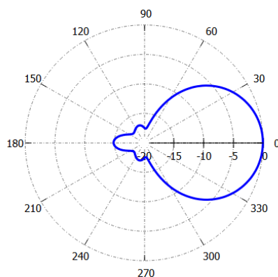
Farfield Directivity 900MHz - H-plane [dB]
