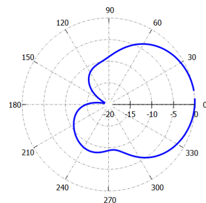
Farfield Directivity 900MHz - V-plane [dB]
