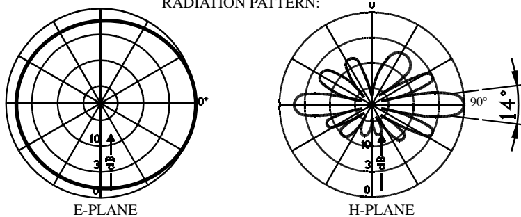
RADIATION PATTERN:
