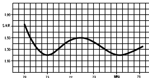
V.S.W.R. CURVE
