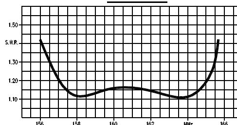
V.S.W.R. CURVE
