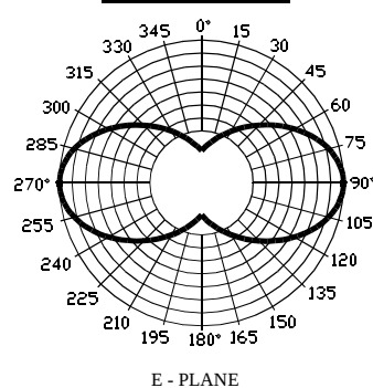
RADIATION PATTERN
