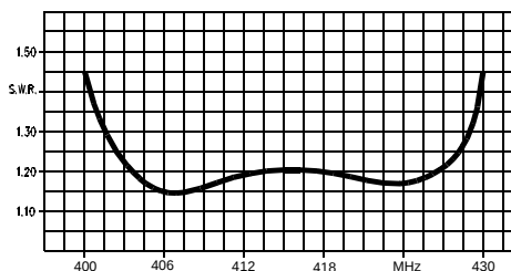
V.S.W.R. CURVE
