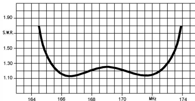
V.S.W.R. CURVE
