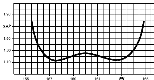
V.S.W.R. CURVE
