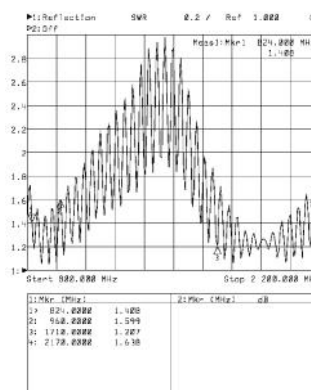
SWR CURVE
