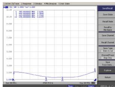
V.S.W.R. CURVE
